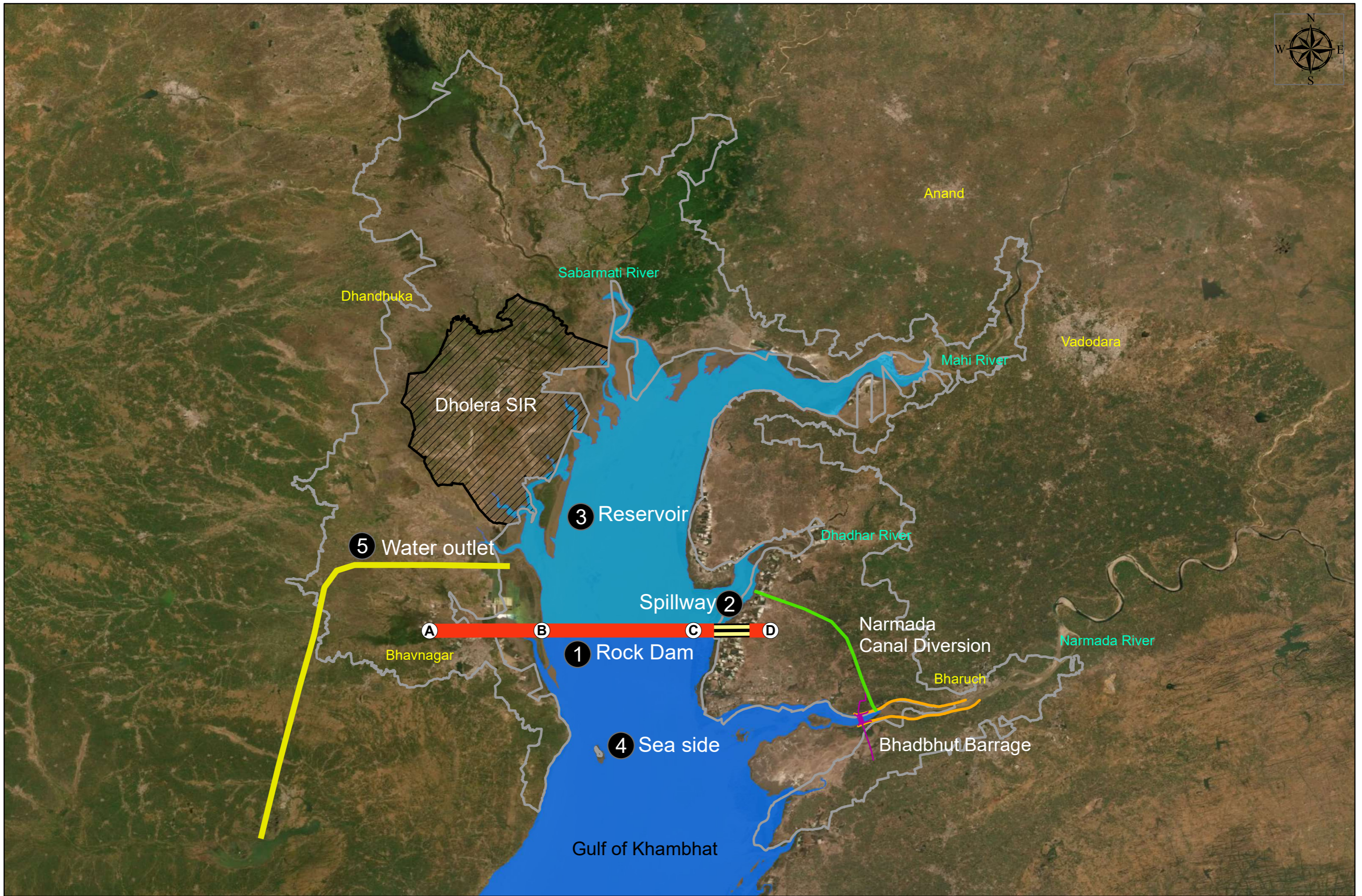
Domains of Instrumentation of Kalpasar Dam
